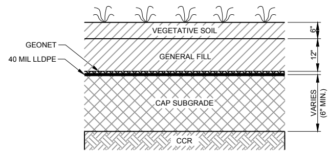
1 6 LLDPE CAP DETAIL NOT TO SCALE
