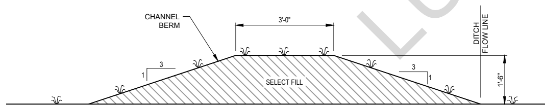
3 6 CHANNEL BERM NOT TO SCALE
