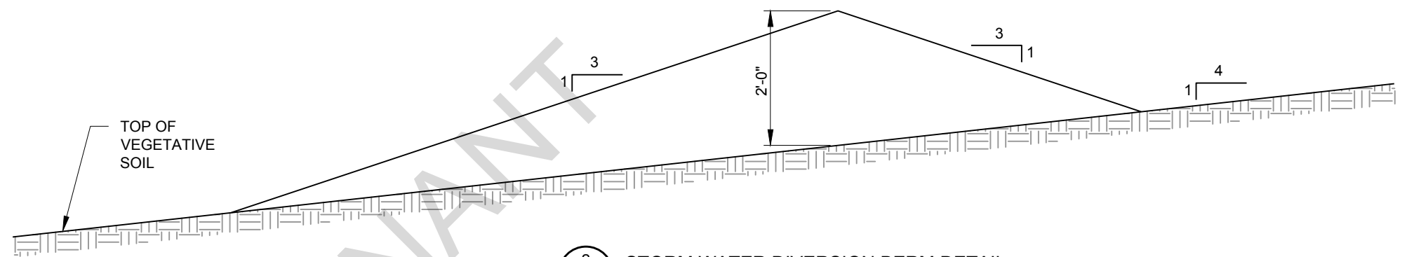
2 6 STORM WATER DIVERSION BERM DETAIL SCALE: 1"= 2'
